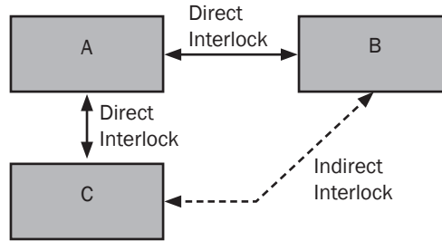
Figure 10. . Illustrative diagram of an indirect interlock
