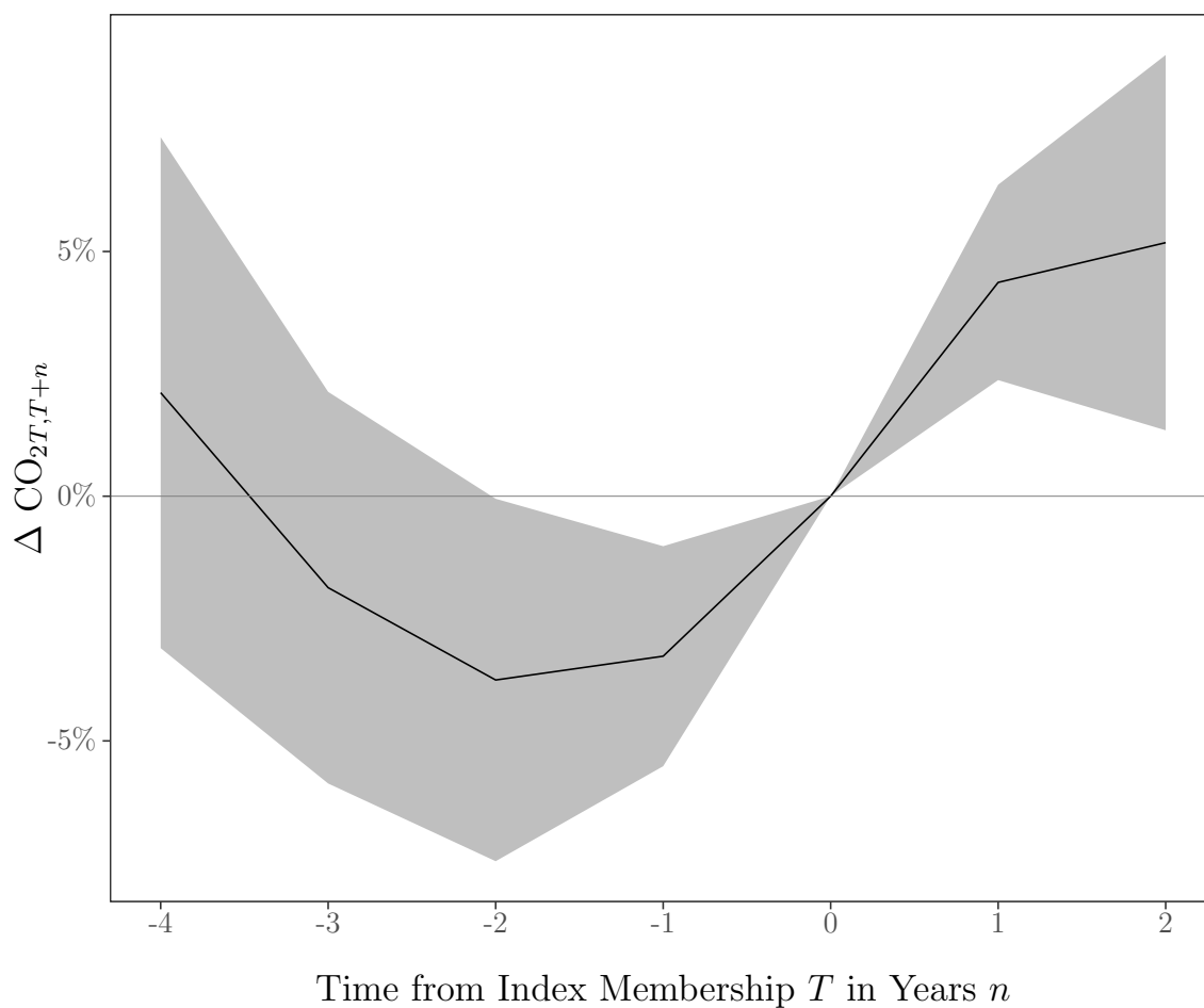
Figure C.5: Inclusion to Index Effect
